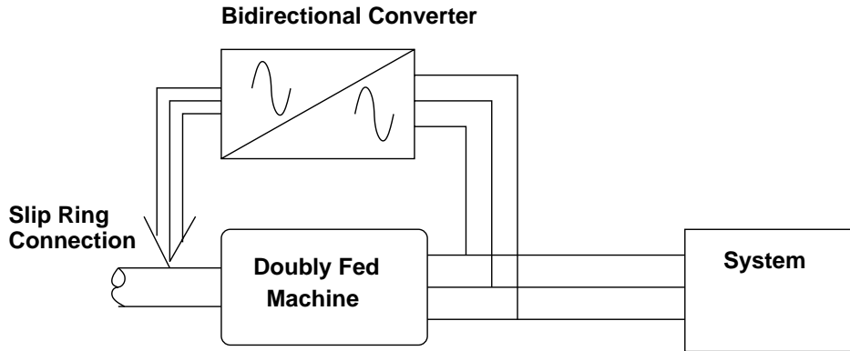
Figure 1: Doubly Fed Machine
