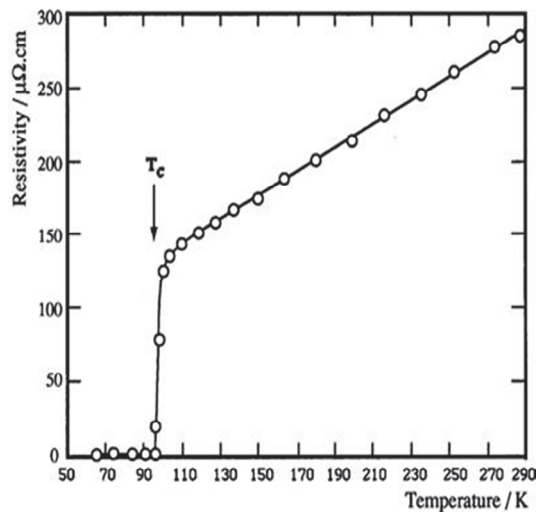
Fig. 8. Temperature and Resistivity of HTS conductor
