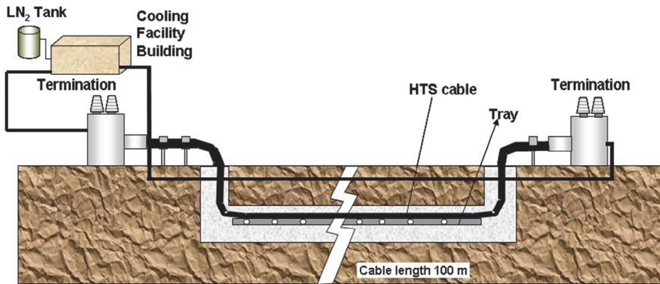
Fig. 4. General conceptual diagram of HTS cable system
