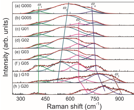
Fig. 9. The the typical spectrum of \text{MgB}_2 consisting of three broad peaks
