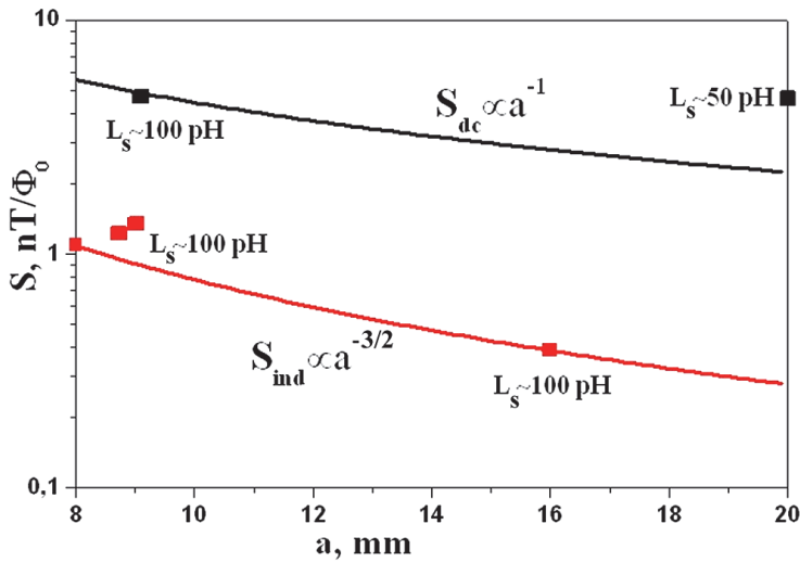
Fig. 9. Flux sensitivity S(\text{nT}/\Phi_0) vs pick-up loop size a(\text{mm}) for direct coupled magnetometers (■, S_{\text{dc}} ) and for the inductively coupled magnetometers with multitrans input coil (■, S_{\text{ind}} ) (Faley et al., 2001).
