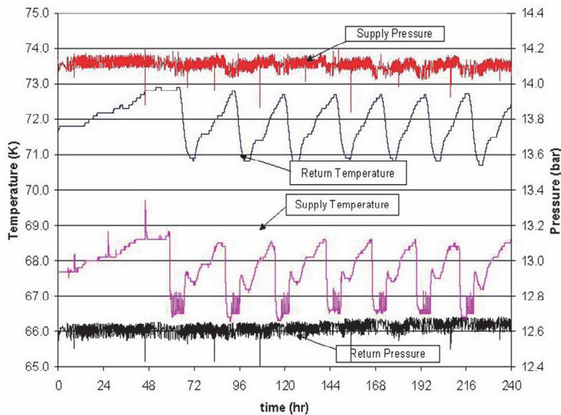
Fig. 9. Inlet and outlet temperature of HTS cable
