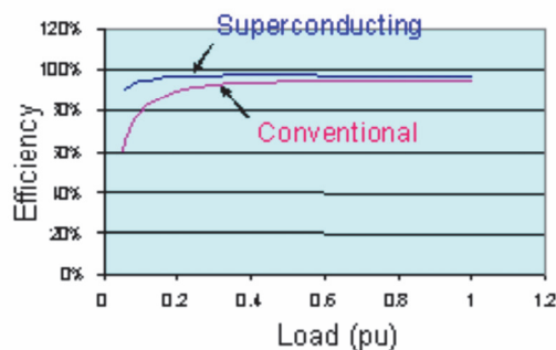
Fig. 24. DSC versus conventional machine efficiency
