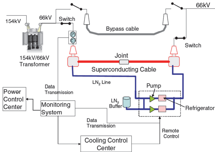
Fig. 7. HTS cable system at Albany project
