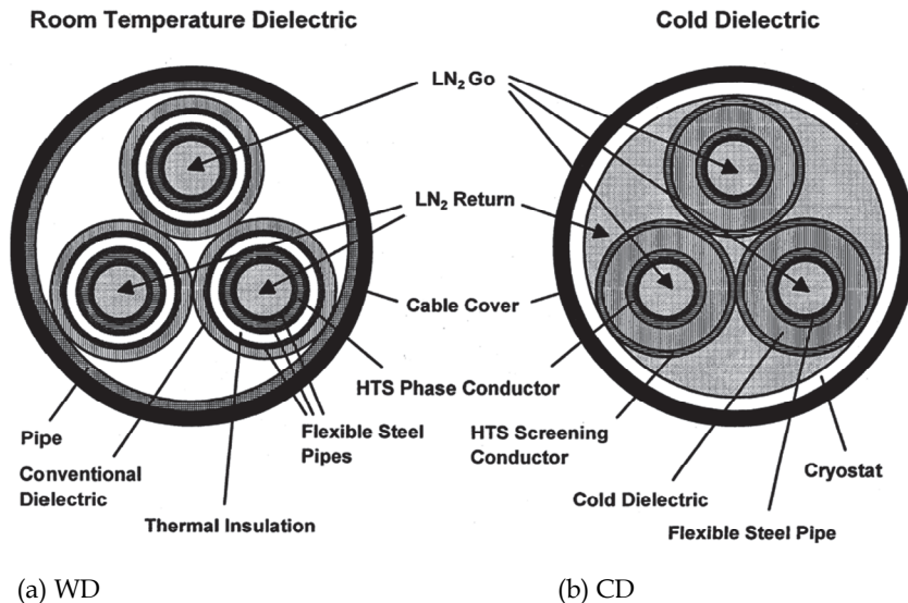
Fig. 3. WD and CD HTS cable
