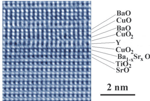
Fig. 2. Cross-sectional HRTEM image of the interface between YBCO and STO films obtained in the [110] direction (Faley et al., 2008).
