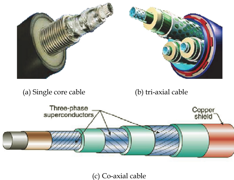
Fig. 5. HTS cable type classified by core
