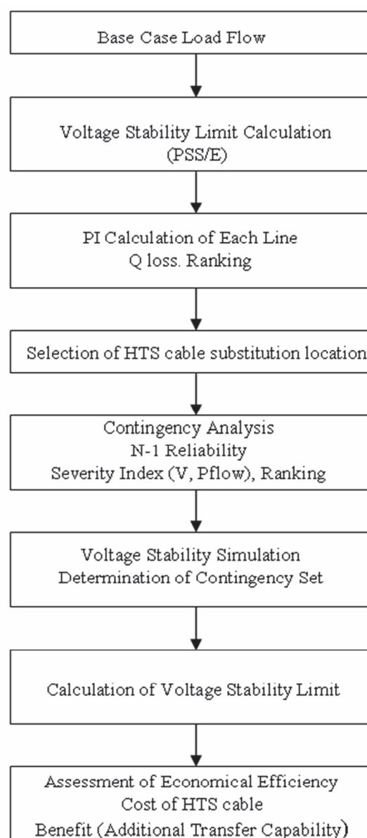
Fig. 26. Analysis procedure of HTS cable application
