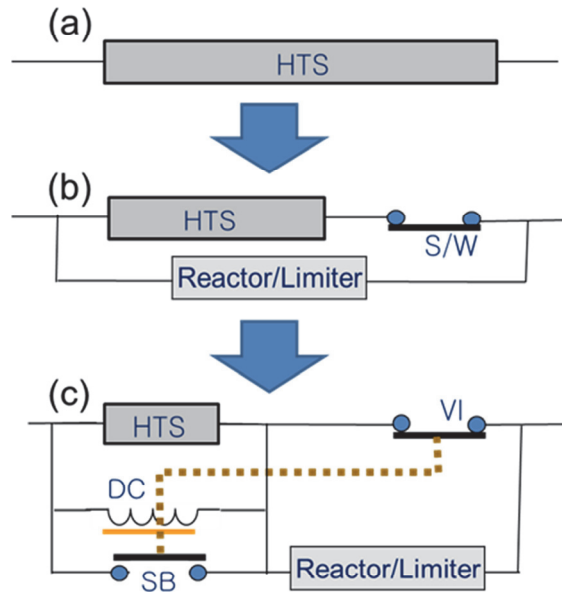
Fig. 19. Design innovation of resistive SFCLs. (a) conventional resistive type, (b) hybrid type with a conventional breaker, (c) hybrid type with a fast switch
