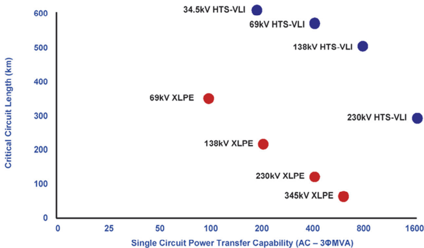
Fig. 2. Comparison of conventional cable to HTS cable
