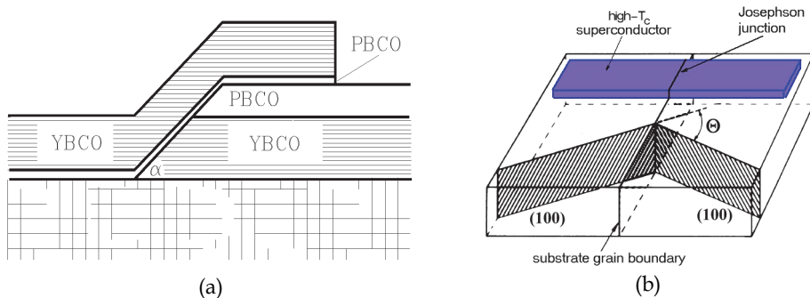
Fig. 8. Schematics of the ramp-type (a) and bicrystal (b) high- T_c Josephson junctions.
