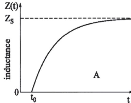
Fig. 16. Characteristics of SFCL impedance
