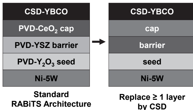
Fig. 1. The schematic of the standard RABiTS architecture.
