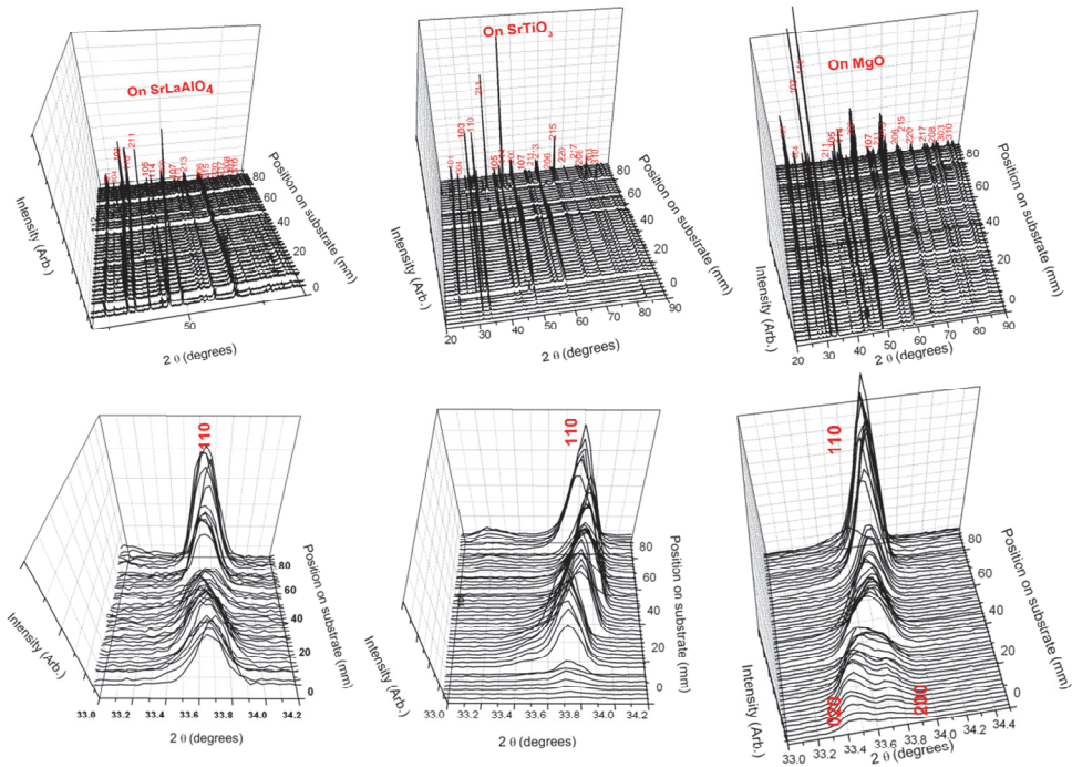
Fig. 6. X-ray diffraction of film library deposited onto three substrates ( \text{SrLaAlO}_4 , \text{SrTiO}_3 and \text{MgO} ). The results (top panel of three) show the peaks can all be indexed to the \text{La}_{214} compound, and in the bottom panel of three the region where peaks sensitive to the tetragonal to orthorhombic phase transition ( [110] - [020/200] ) are found.
