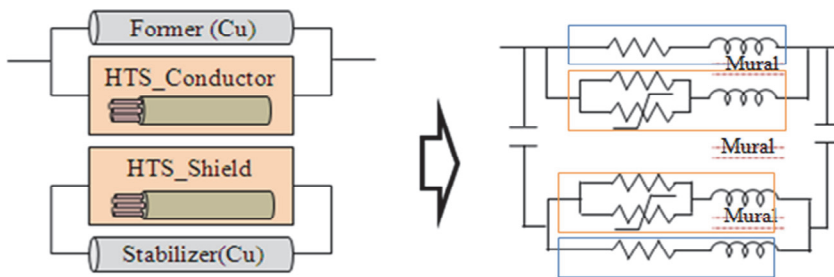
Fig. 9. CD type HTS cable modeling
