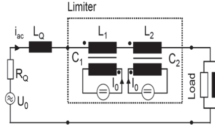
Fig. 17. Saturable core type SFCL conceptual circuit
