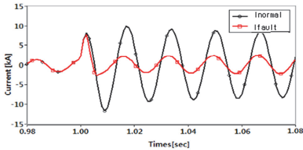
Fig. 22. Simulation result of SFCL dynamics
