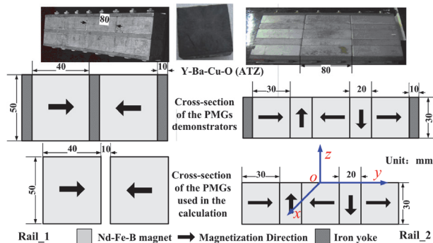
Fig. 4. Photos of the Y-Ba-Cu-O sample and magnetic rail demonstrators and associated schematic drawings of magnetic rail's cross sections.
