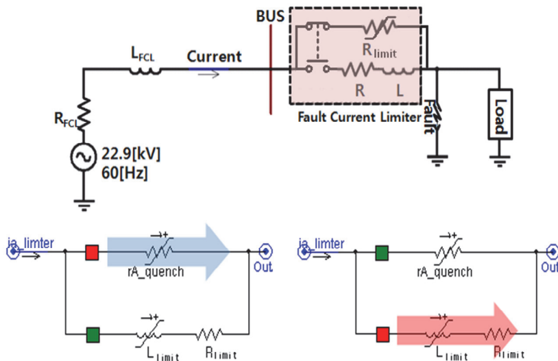
Fig. 21. SFCL sample system
