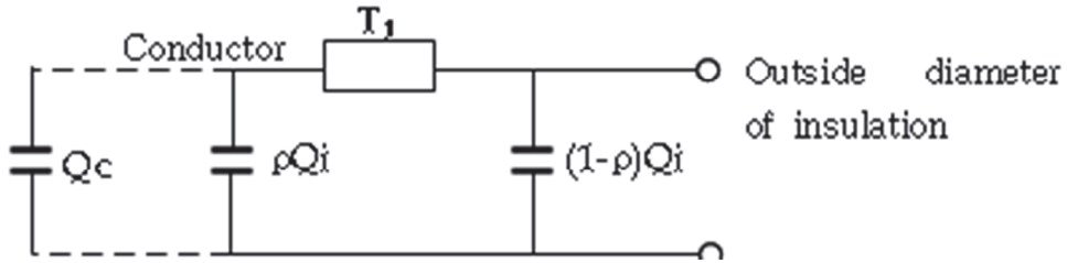
Fig. 13. Equivalent heat transfer circuit of HTS cable
