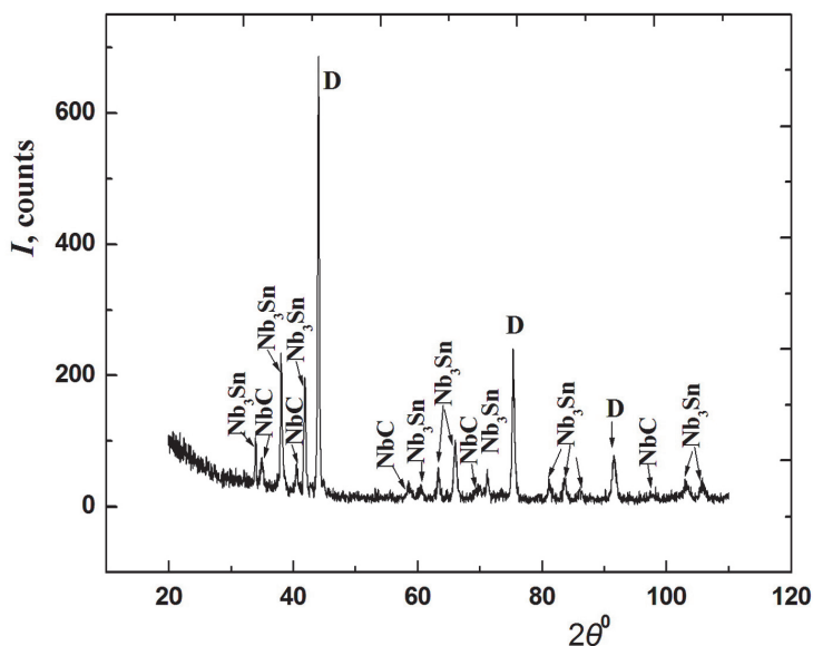
Fig. 16. X-ray diffraction pattern of (50% \text{Nb}_3\text{Sn} + 50% micropowder diamond) sample sintered at P = 7.7 GPa, T = 1625 K; \text{D} – reflections of diamond, \text{NbC} – reflections of niobium carbide.
