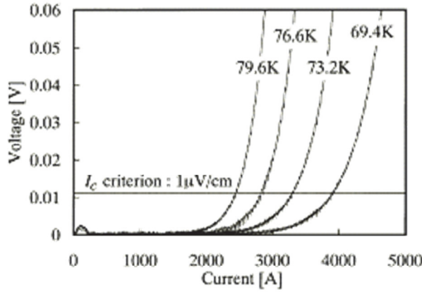
Fig. 12. V-I curve of 66kV HTS cable
