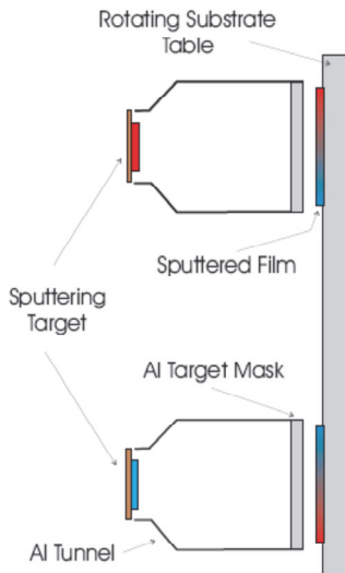
Fig. 5. Schematic side view (left) and actual (right) front-view image of the sputtering machine set-up with linear-in (at 4:00) and linear-out (at 12:00) masks placed in front of each target (color on-line).
