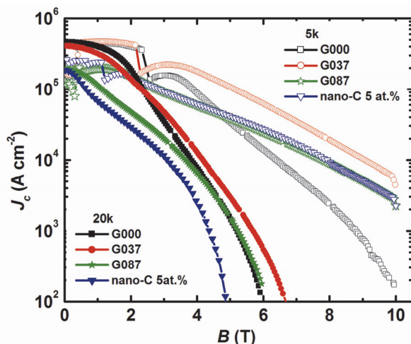
Fig. 5. Magnetic critical current density as a function of magnetic field at 5 K and 20K for with and without graphene doped bulk samples. 5 at% nano-C doped sample for a comparable result at the same sample preparation route (Xu, X. et al., 2010).
