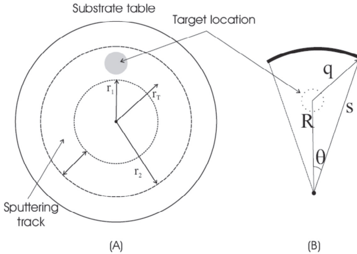
Fig. 3. Vectors defining important locations on the substrate table (A) and those needed to define the target mask (B).
