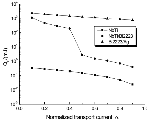
Fig. 14. MQE Q_E of three types of conductors
