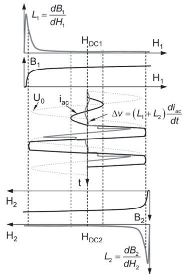
Fig. 18. Saturable core type characteristics
