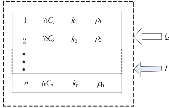
Fig. 5. Overview of a composite conductor with longitudinally flowing heat Q and current I
