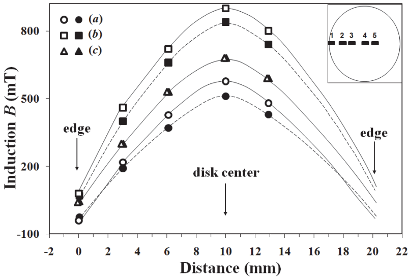
Fig. 7. Local induction B vs. Hall probe location measured on the surface of the sample in the experiments (a), (b) and (c): 2 min (open symbols) and 100 min (full symbols) after placing the sample in the final position. The solid and dashed lines serve as a guide for the eye. The inset shows the location of Hall probes.
