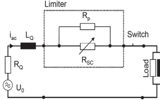
Fig. 15. R-type and L-type SFCL conceptual circuit
