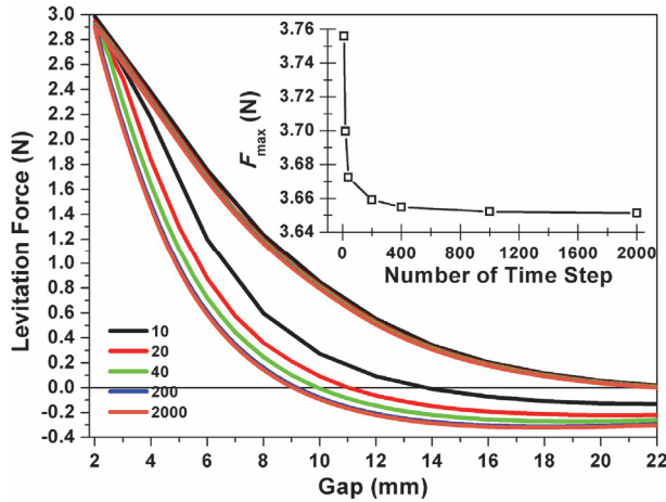
Fig. 3. Levitation force versus gap with different number of time step and the maximum levitation force F_{\max} as a function of the number of time step (inset).
