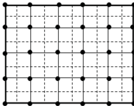
Figure 7-4: Finite volume grid and cells.
